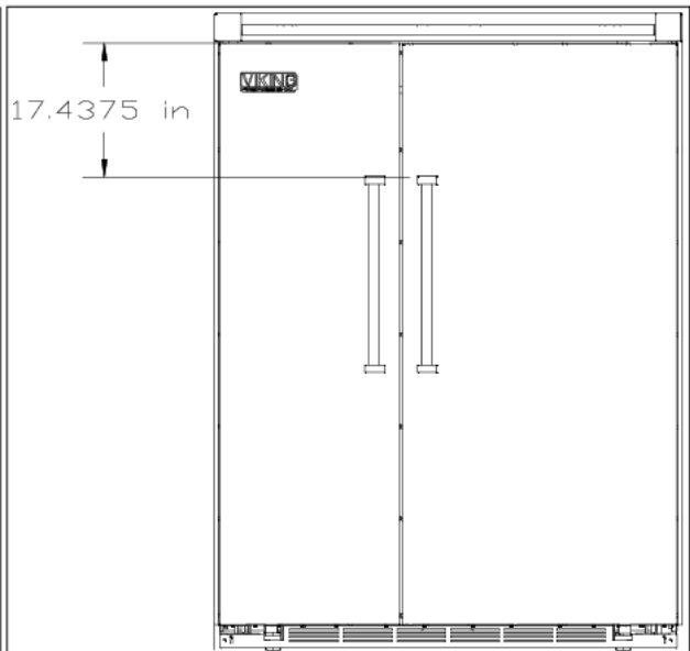
FIGURE 2-CURRENT HANDLE LOCATION DIMENSION
