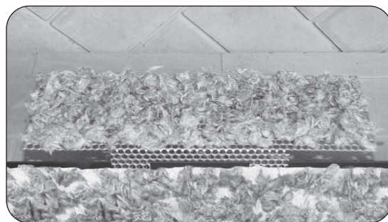
Fig. 22-2 Cover screen with embers
