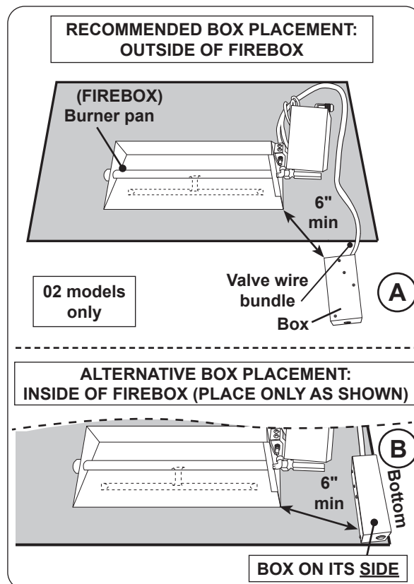
Fig. 18-1 Box placement (if applicable)
