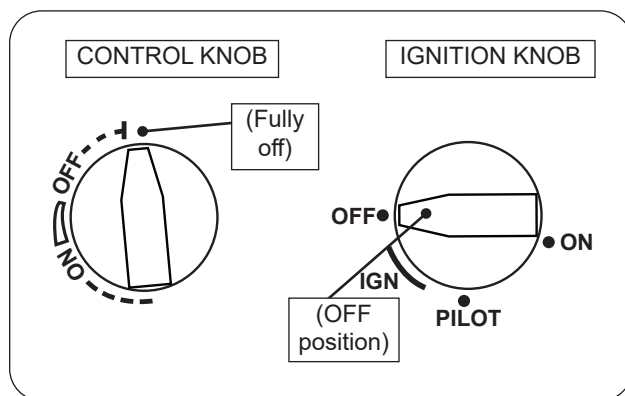
Fig. 33-2 Manual shut down
