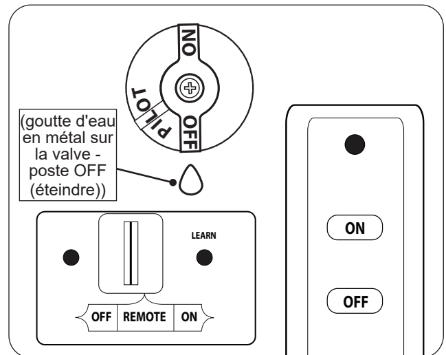
Fig. 49-2 Remote shut down
