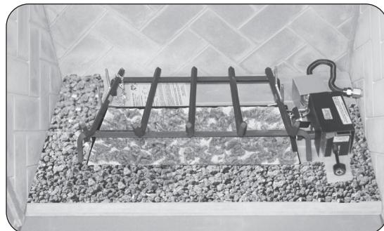
Fig. 22-3 Place grate
