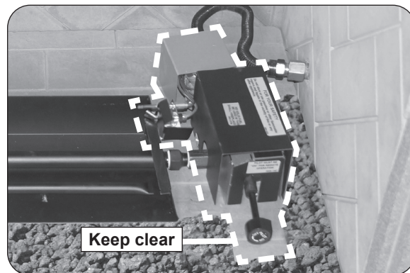
Fig. 20-3 Proper lava media placement
