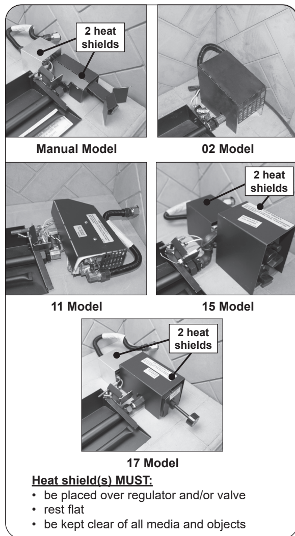
Fig. 20-1 Place heat shield(s)
