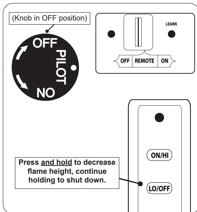
Fig. 37-2 Remote shut down
