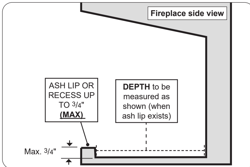
Fig. 8-1 Ash lip/recess detail
