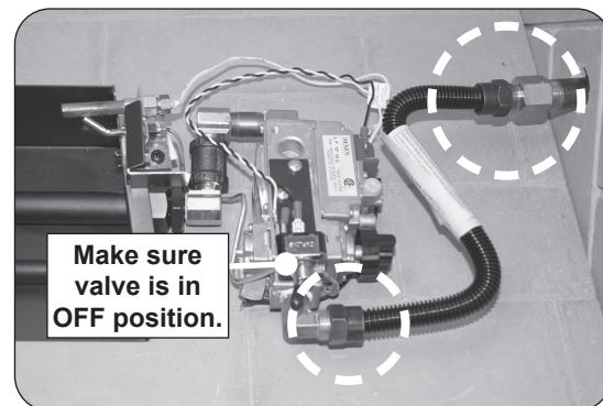
Fig. 17-3 Perform leak test
