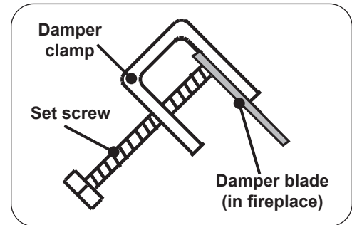
Fig. 11-1 Damper clamp detail
