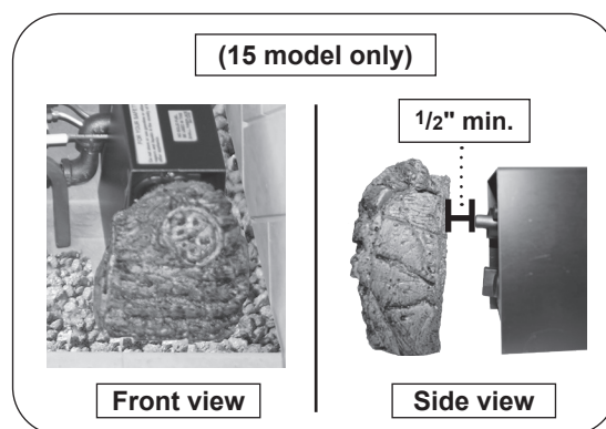
Fig. 22-4 Place wood chip (if applicable)
