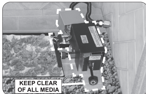
Fig. 21-4 Keep pilot, valve, & shield(s) clear
