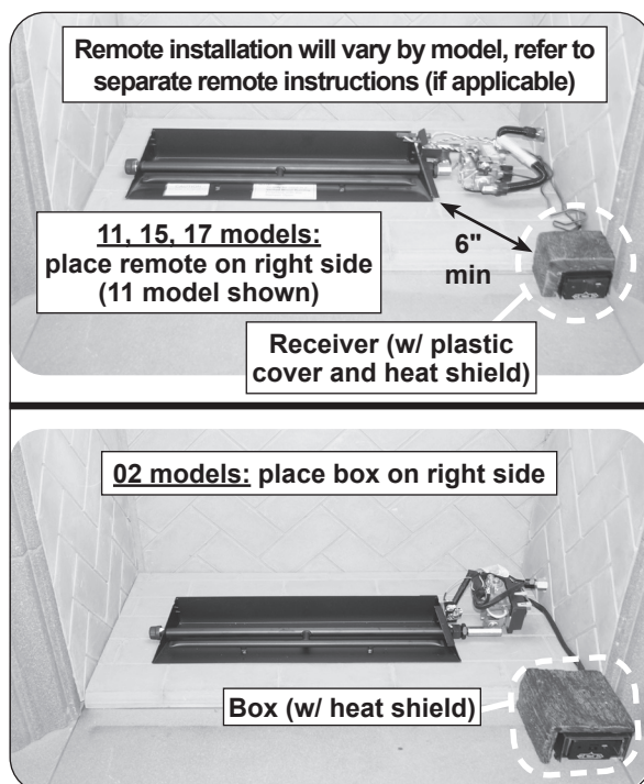
Fig. 18-2 Install remote receiver and heat shield (as applicable)
