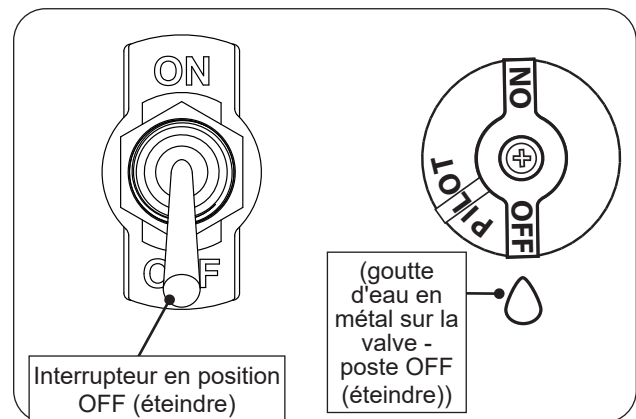
Fig. 48-2 Manual shut down
