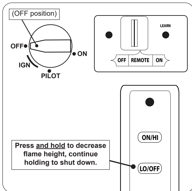
Fig. 34-2 Remote shut down
