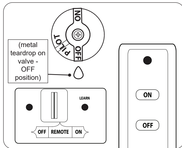
Fig. 31-2 Remote shut down
