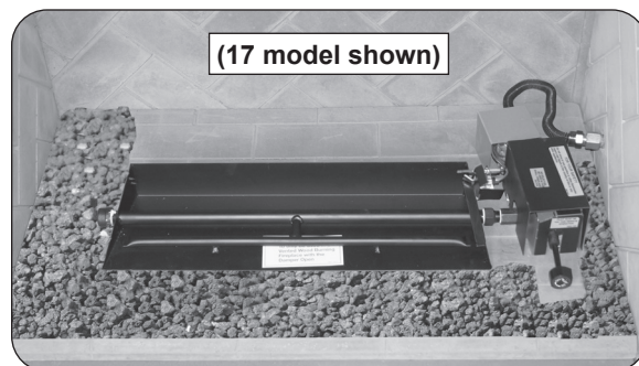
Fig. 20-2 Place lava media (if option purchased)
