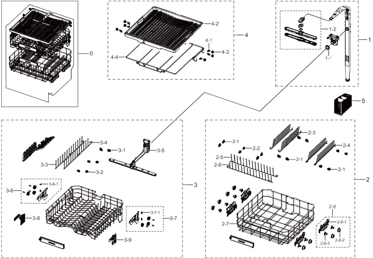
Assy Case Parts List & Assy Basket and Duct
