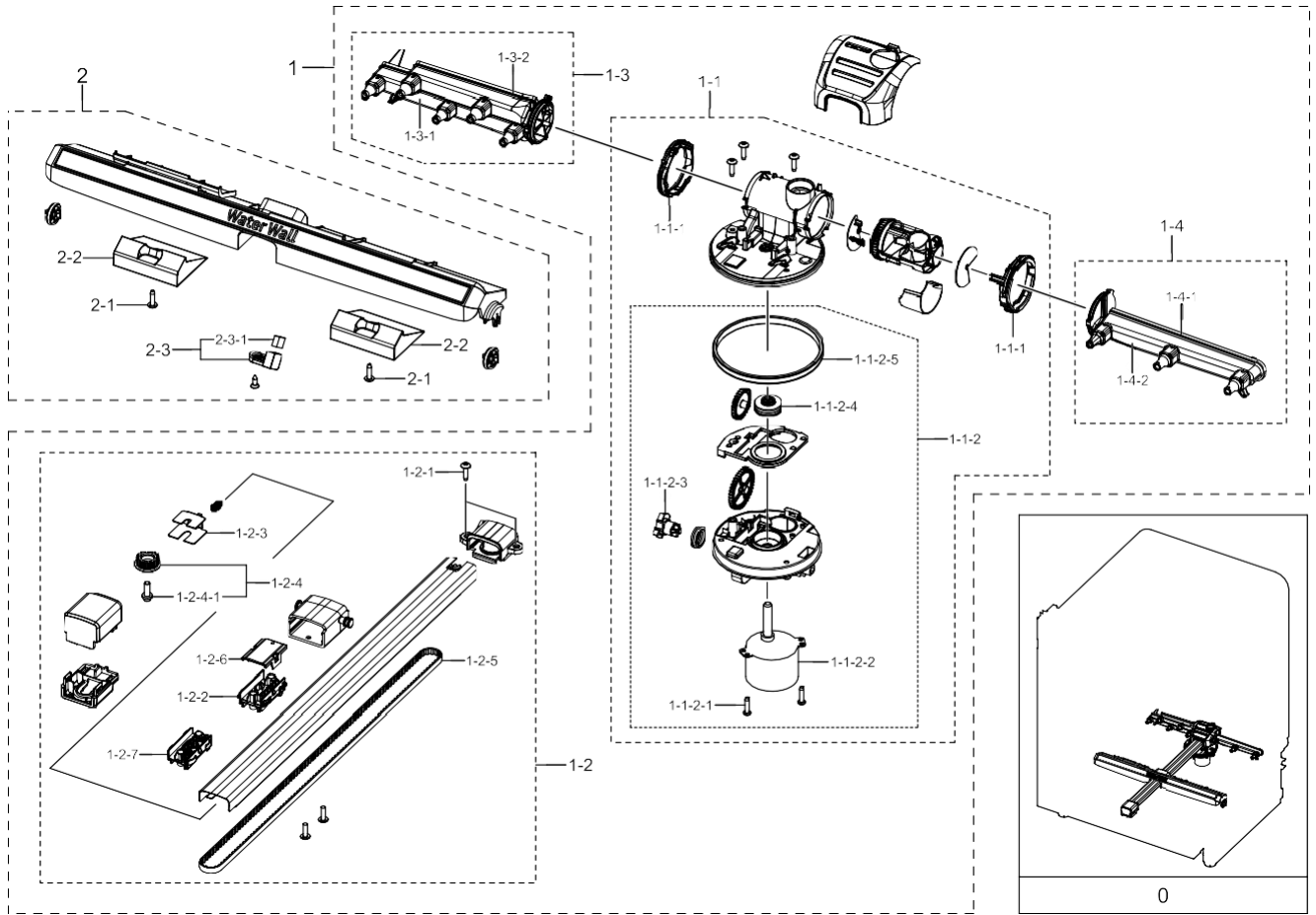
Assy Case Parts List / Assy Motion & Vane
