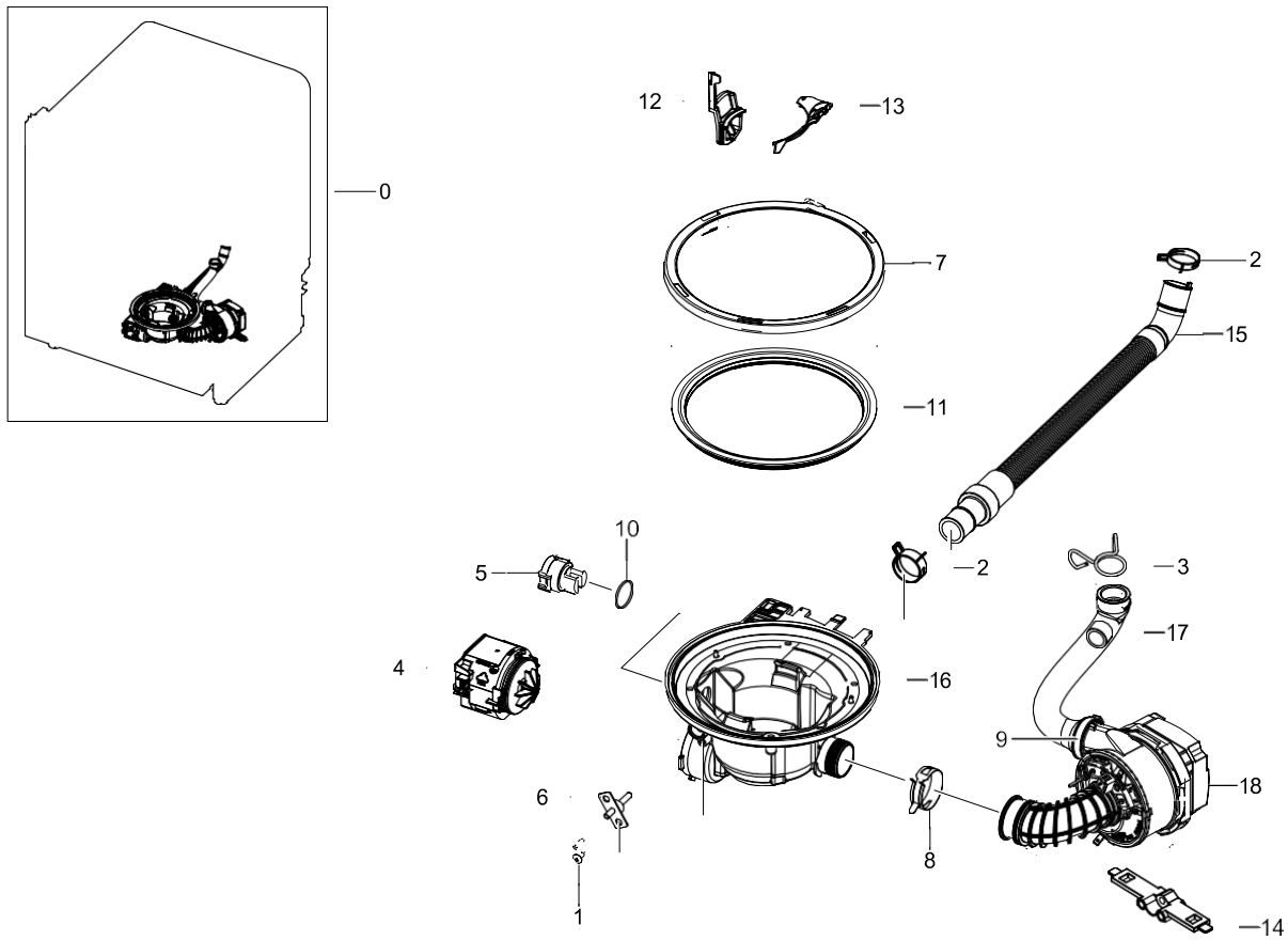
Assy Sump Parts List
